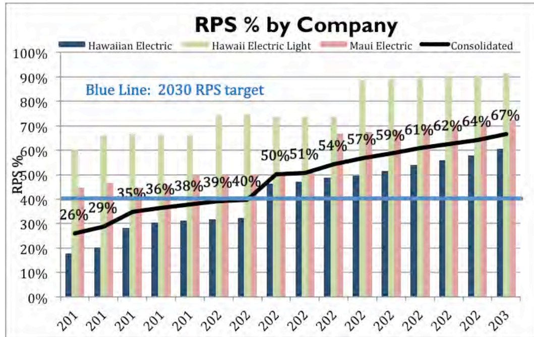
Figure 5-1. Consolidated RPS of Hawaiian Electric Companies' Preferred Plans
