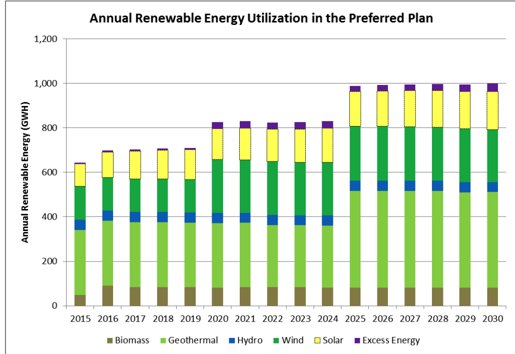
Figure 5-6. Total System Renewable Energy
