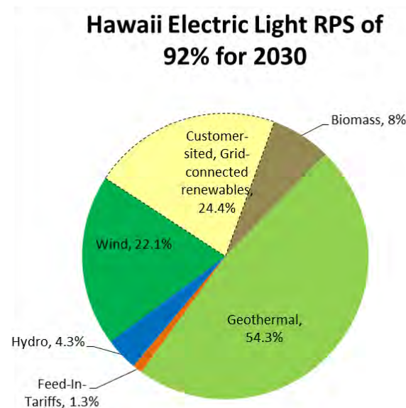
Figure 5-2. Source of Renewable Energy used in the 2030 RPS for Hawai'i Electric Light Preferred Plan
