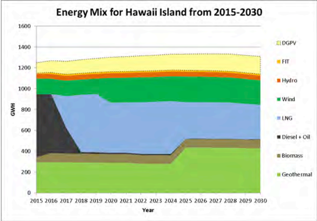
Figure 5-5. Annual Energy Mix of Hawai'i Electric Light Preferred Plan
